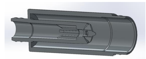
Figure 2: Section view of molded test part.
